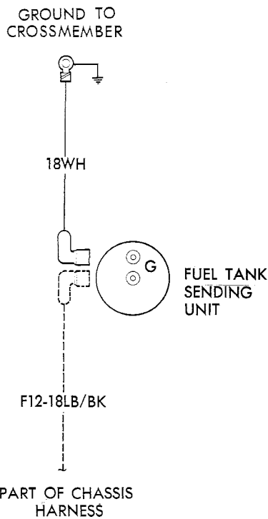
WIRING DIAGRAM-IN-CAB FUEL TANK
