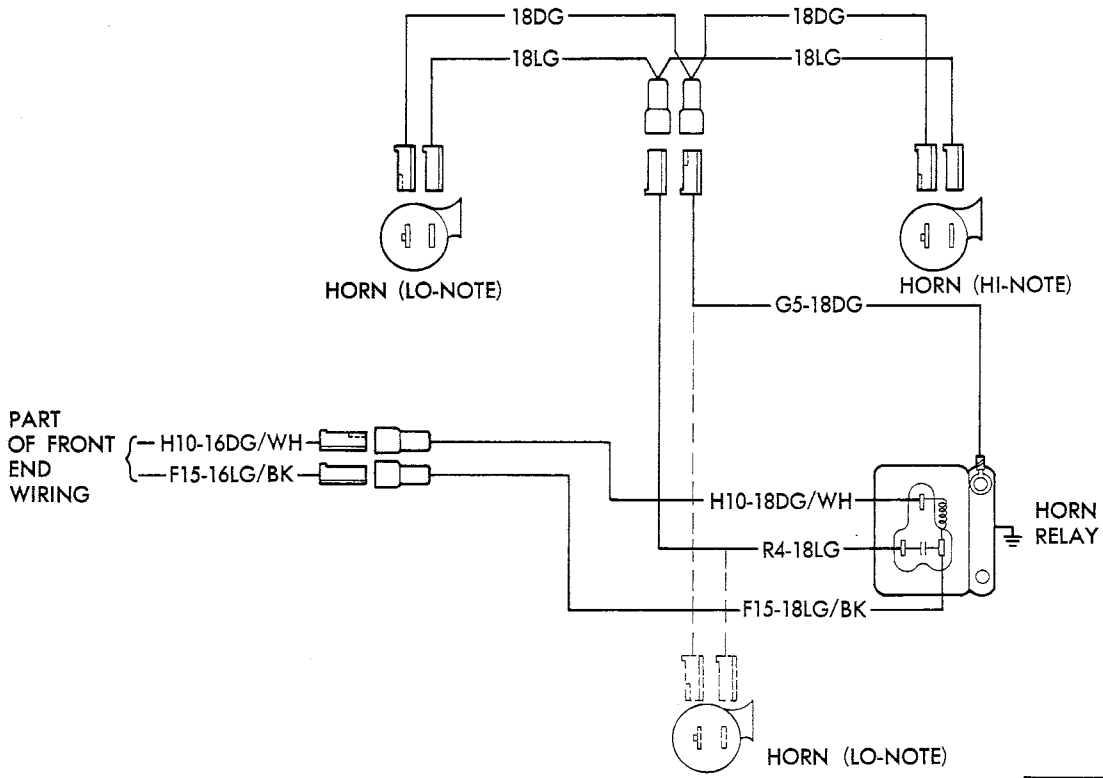
HORN WITH RELAY SINGLE AND DUAL (TILT COLUMN)
