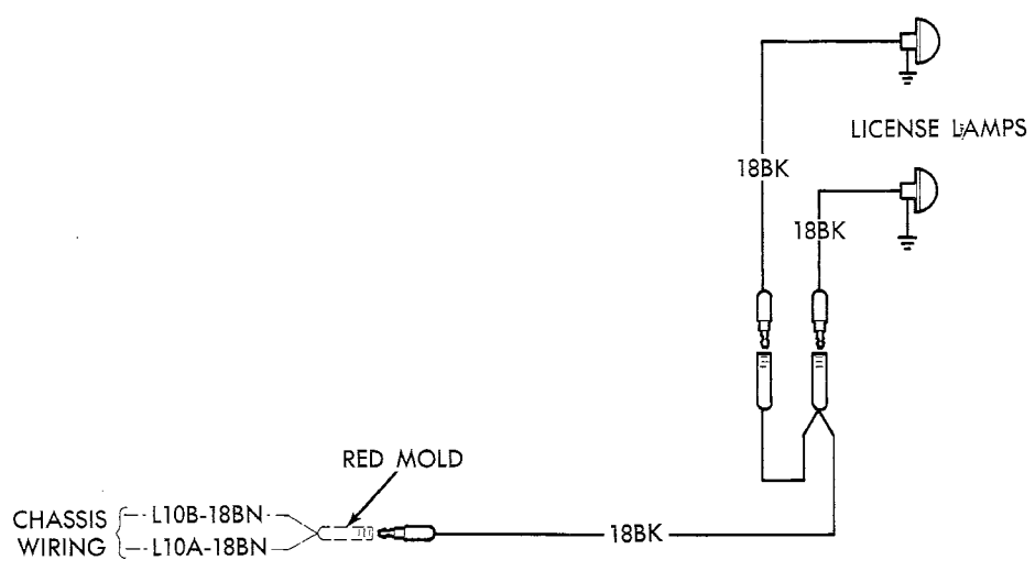
CLEARANCE, IDENTIFICATION AND SIDE MARKER LAMPS
