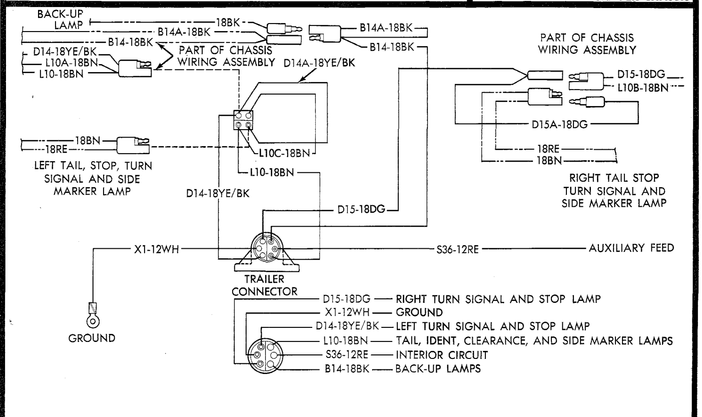
WIRING DIAGRAM - TRAILER TOWING
